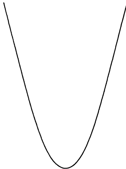
Figure 5: A self-expanding curve
