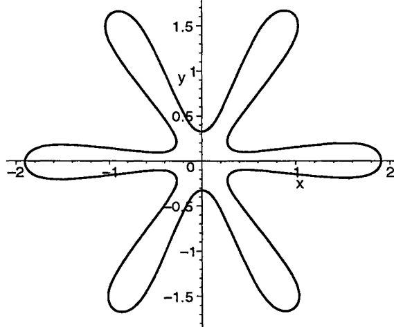
Figure 8: n = 2, p = 17, q = 35
