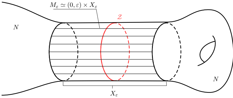
Figure 1.1. Tubular neighborhood of the singular region.
