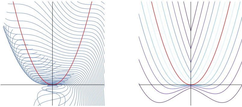
Figure 3.1. Some metric properties of the almost-Riemannian structure (3.1). Left: geodesics satisfying the necessary condition for minimality from \mathcal{Z} (red parabola) and starting at points of \mathcal{Z} with x > 0 . Numerical evidence suggests that they are minimizing until they cross the vertical axis. Right: Level sets of the distance from \mathcal{Z} .
